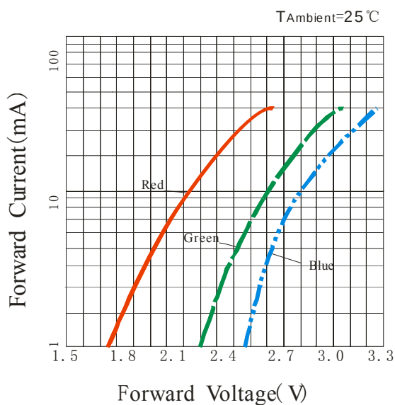
Volt-Ampere Characteristics
