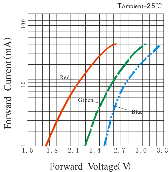
Volt-Ampere Characteristics
