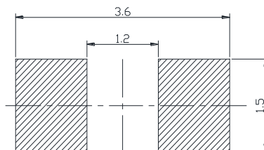
推荐焊盘尺寸 Recommended Soldering Pad
