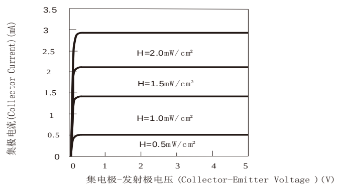
Collector Current VS Collector-Emmitter Voltage
