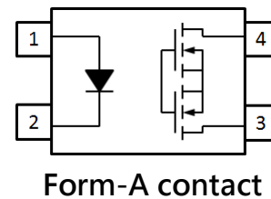
Solid State Relay
