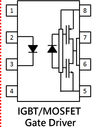
IGBT Gate Driver
