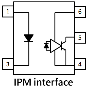
IPM
