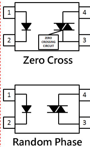
Triac Output
