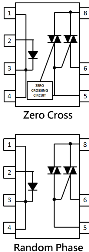
Power Triac
